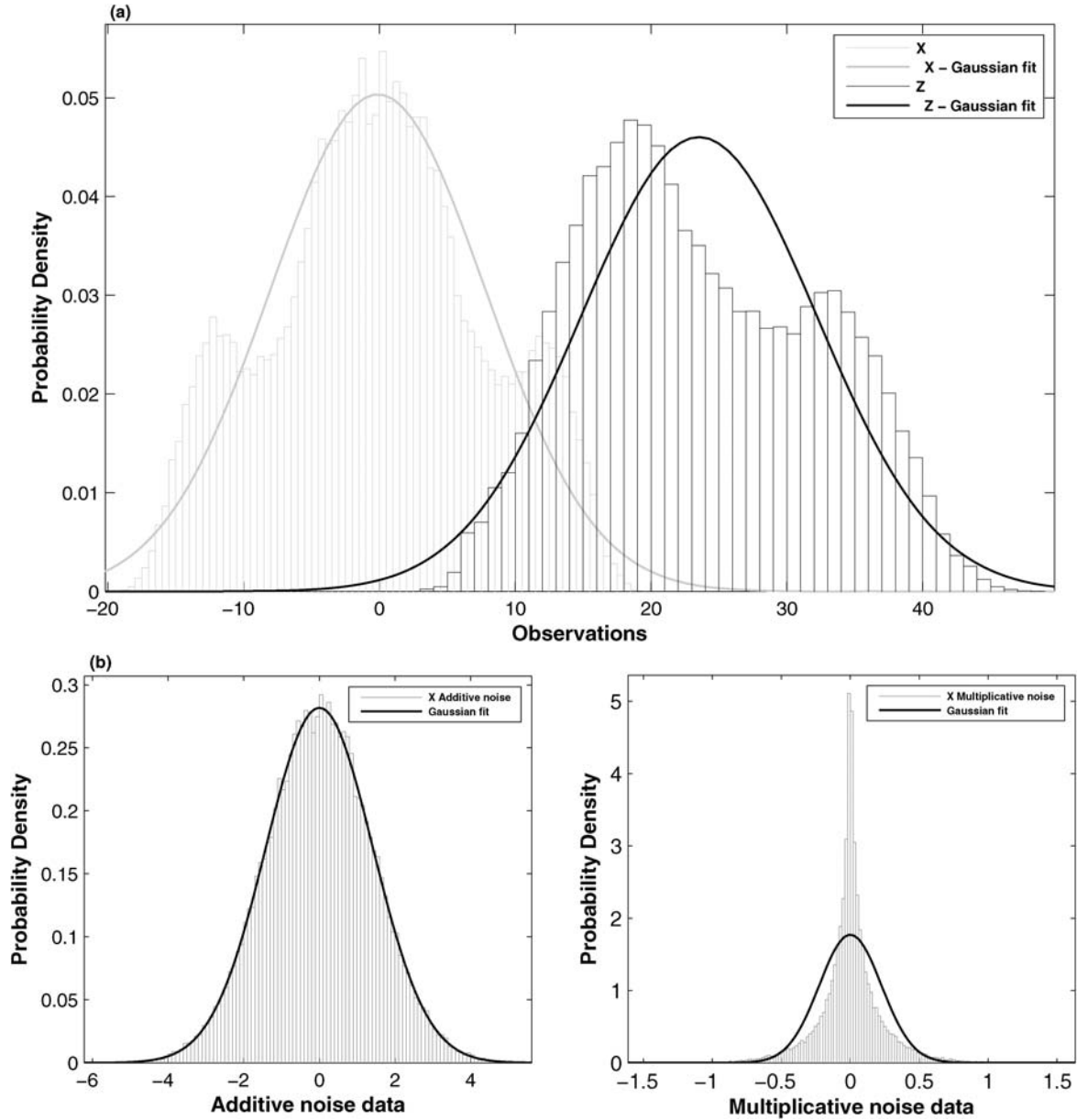
Figure 1. (a) Observation distribution: gray - X, and black - variable Z. (b) Noise distributions for X: (left) additive noise, (right) multiplicative noise; solid curves represent corresponding Gaussian fits.
