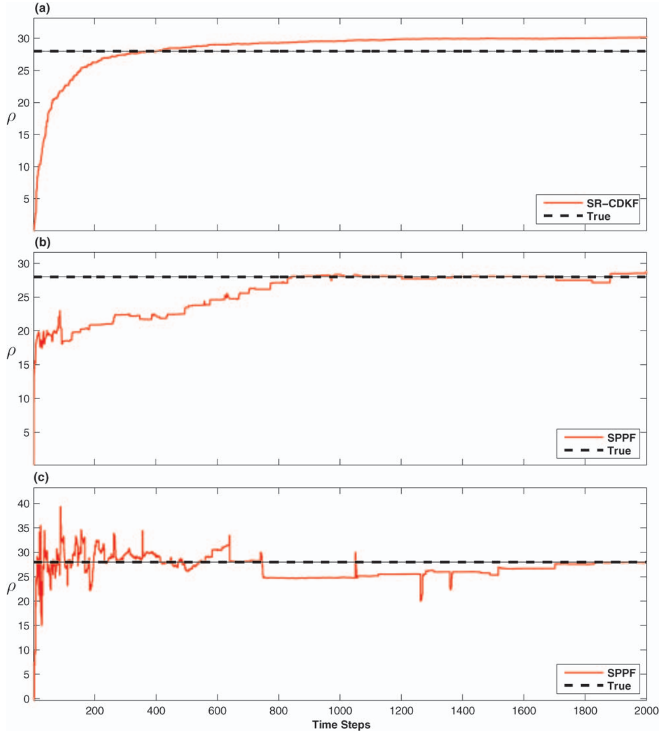
Figure 3. Lorenz '63 model: (a) SR-CDKF and (b) SPPF using 100 particles. (c) SPPF with a higher multiplicity factor of 0.2. True \rho - dashed line, estimated \rho - solid red line.
