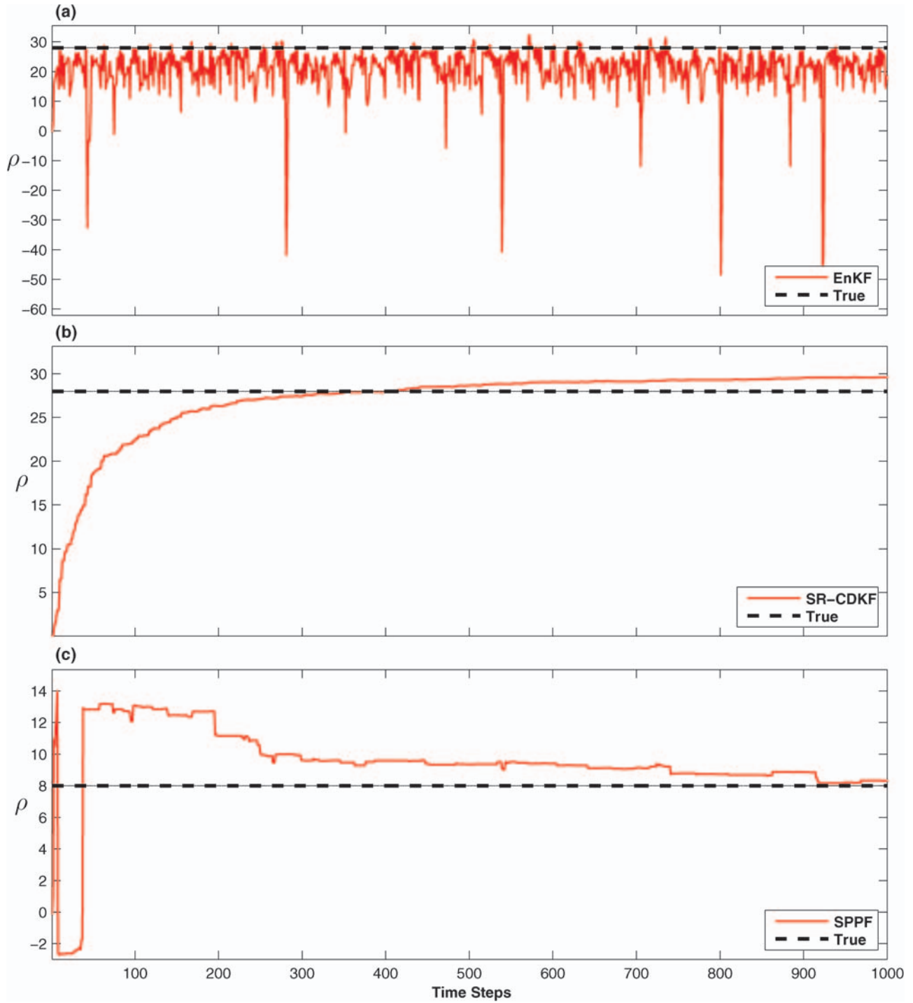
Figure 2. Lorenz '63 model: (a) EnKF and (b) SR-CDKF, and (c) SPPF with 100 particles. True \rho - dashed line, estimated \rho - solid red line.
