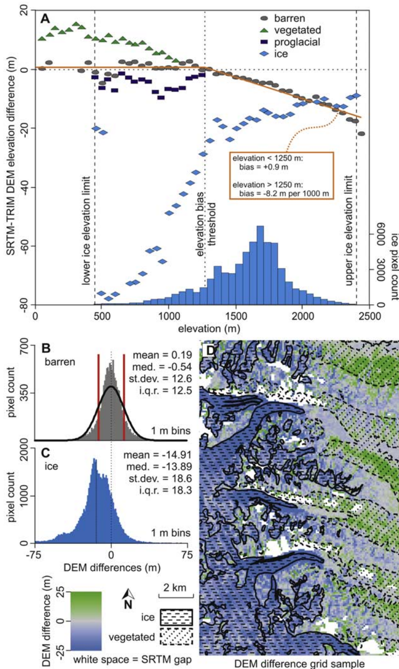
Figure 2. (a) SRTM-TRIM elevation differences for NTDB sheet 103P13 (A in Figure 1) over barren, vegetated, proglacial, and glacierized terrain. Histogram shows the altitudinal distribution of ice cover. Piecewise linear adjustment for bias correction shown by red line. (b) Histogram and statistics of elevation deviations for barren terrain with interquartile range (vertical red lines) and Gaussian fit (black line). (c) Histogram and statistics of elevation differences for ice covered terrain. (d) Surface elevation change over moderately glacierized terrain.
