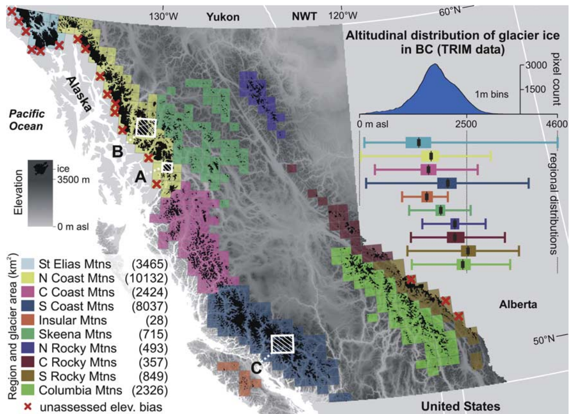
Figure 1. Hypsometric shading shows the relief and geographic extent of BC. Regionally color coded areas delimit the 1:50 k NTDB maps which contain glaciers (dark fill). Hatched box A is the area illustrating terrain biases (Figure 2). Hatched boxes B and C are the Andrei and Lillooet icefield areas (regions of SRTM-NTDB analysis). Histogram shows the altitudinal distribution of glacial ice based on TRIM data with underlying box plots indicating the total range (whisker), interquartile range (box), and median (black line) ice elevation by region.
