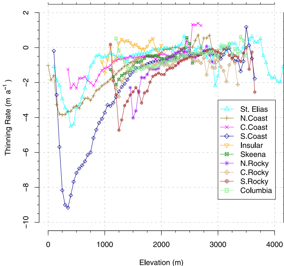
Figure 3. Observed glacier thinning rates vs. altitude for the SRTM-TRIM data for the different regions defined in Figure 1.
