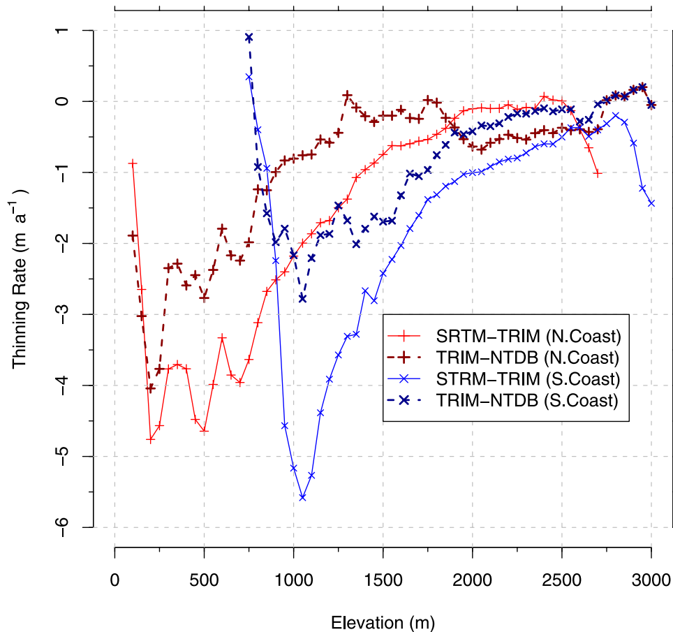
Figure 4. Thinning rates vs. elevation for the SRTM-TRIM and TRIM-NTDB data for the Andrei and Lillooet icefields (B and C in Figure 1).
