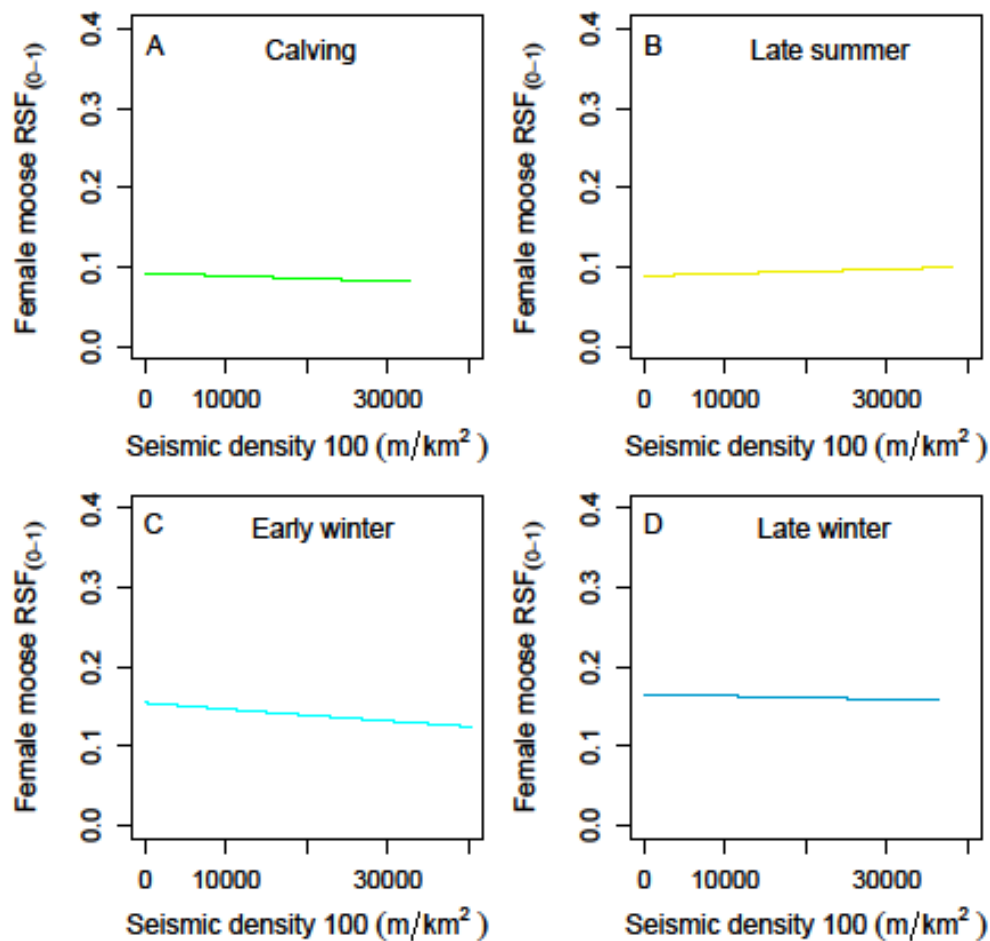
Figure 15. Relative predicted probability of selection of tree bog vegetation class (most frequently used vegetation class by caribou) by female moose as a function of seismic line (seismic) density for each season. The number (100) following seismic density in the x-axis label indicates the buffer in m (see text) of the best-supported univariate seismic density model determined via AIC c for each season.
